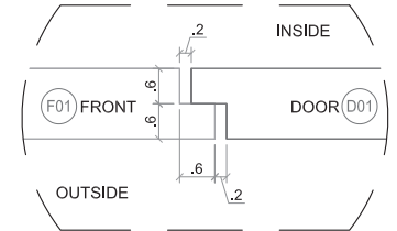
TYPICAL JOINT / DOOR WITH FRONT PANEL
