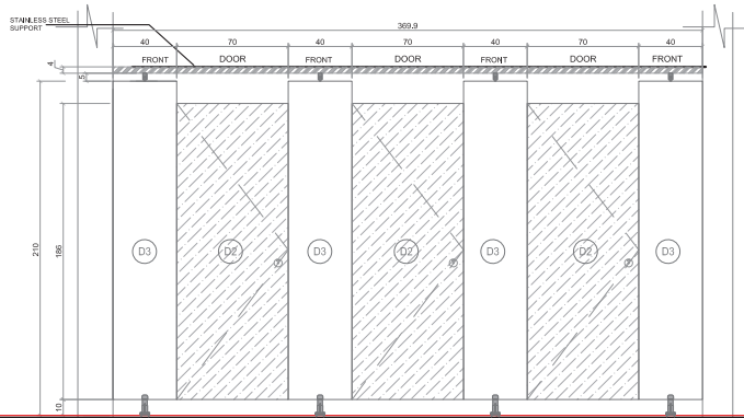
W.C. - ELEVATION CUBICLES
