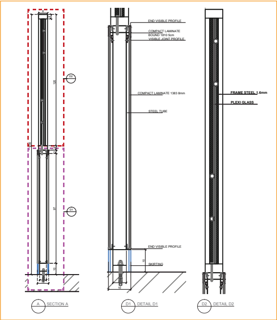
SECTION A
