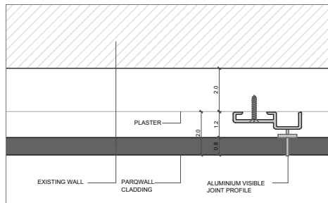
F VISIBLE PROFILE-INTERIOR PROFILE
