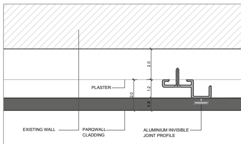
E INVISIBLE PROFILE-INTERIOR PROFILE
