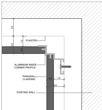
A INVISIBLE CORNER-INTERIOR PROFILE
