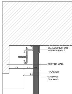
C END VISIBLE PROFILE-INTERIOR
