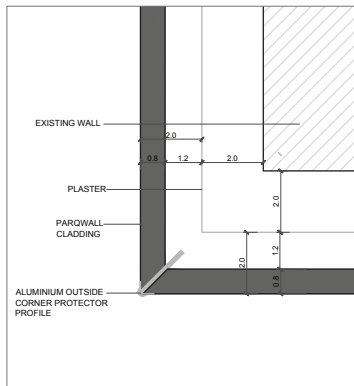
B OUTSIDE CORNER-INTERIOR PROFILE
