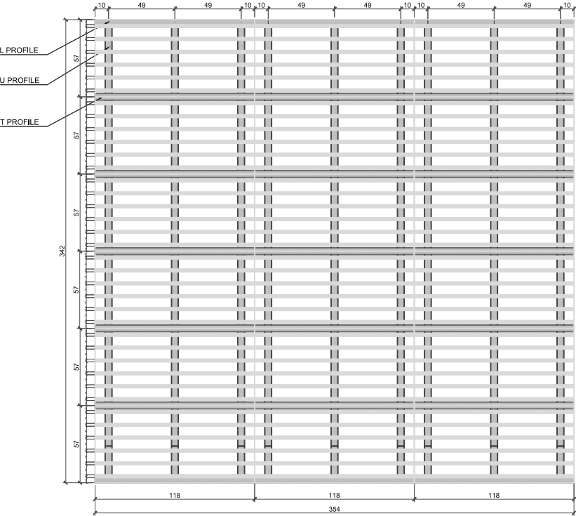
PLAN CEILING LAYOUT-STRUCTURE 1:20 @ A3 MTS
