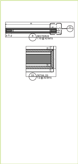
SECTION B
