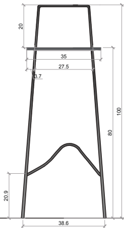
BACK ELEVATION
